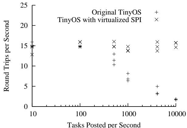
Figure 7. Posting tasks interferes with radio reception in the standard TinyOS kernel
